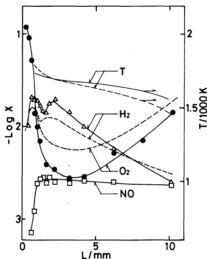
Fig. 6. Effects of \text{CH}_3\text{NH}_2 addition on the profiles of concentrations of \text{H}_2 and \text{O}_2 , and temperature in a free-burning methanol-air flame. The dashed lines and the solid lines denote the flame without and with addition of 0.58% \text{CH}_3\text{NH}_2 .
